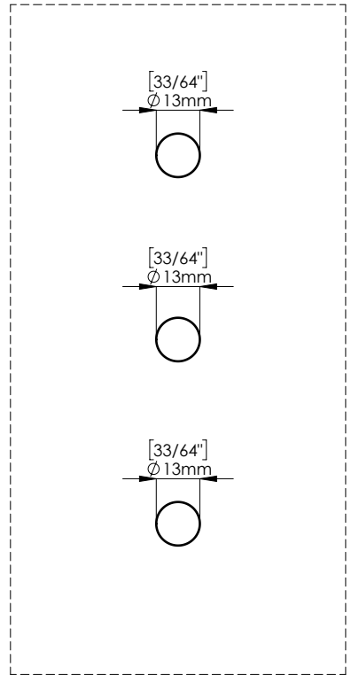
GLASS CUTOUT
