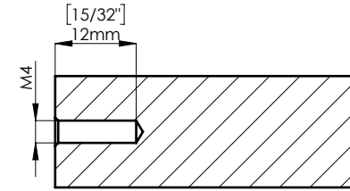
SECTION L-L
