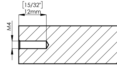
SECTION L-L
