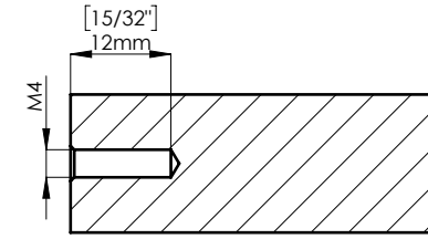
SECTION L-L
