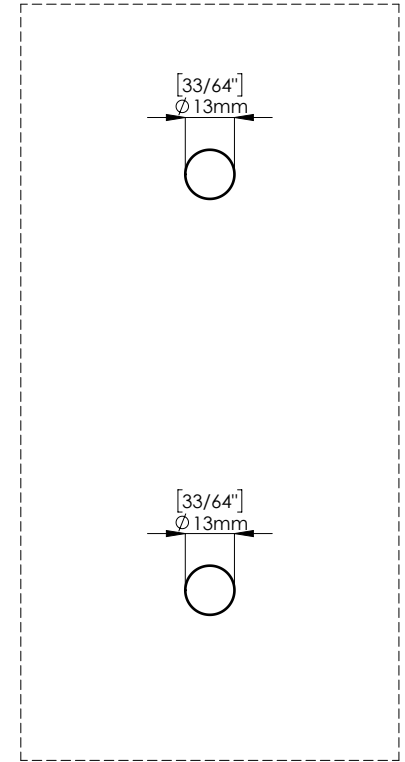
GLASS CUTOUT
