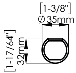
TUBE DETAIL
