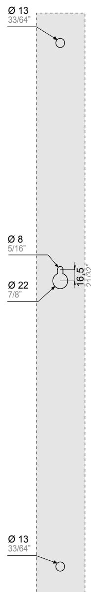
DOUBLE GLASS DOOR PREP (FOR SPACER KITS)
