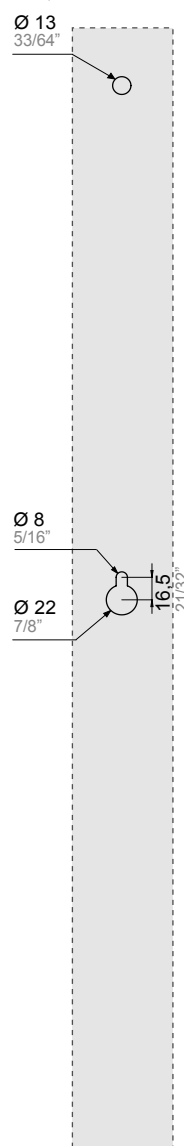
DOUBLE GLASS DOOR PREP (FOR SPACER KITS)
