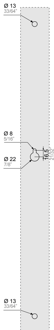
DOUBLE GLASS DOOR PREP (FOR SPACER KITS)
